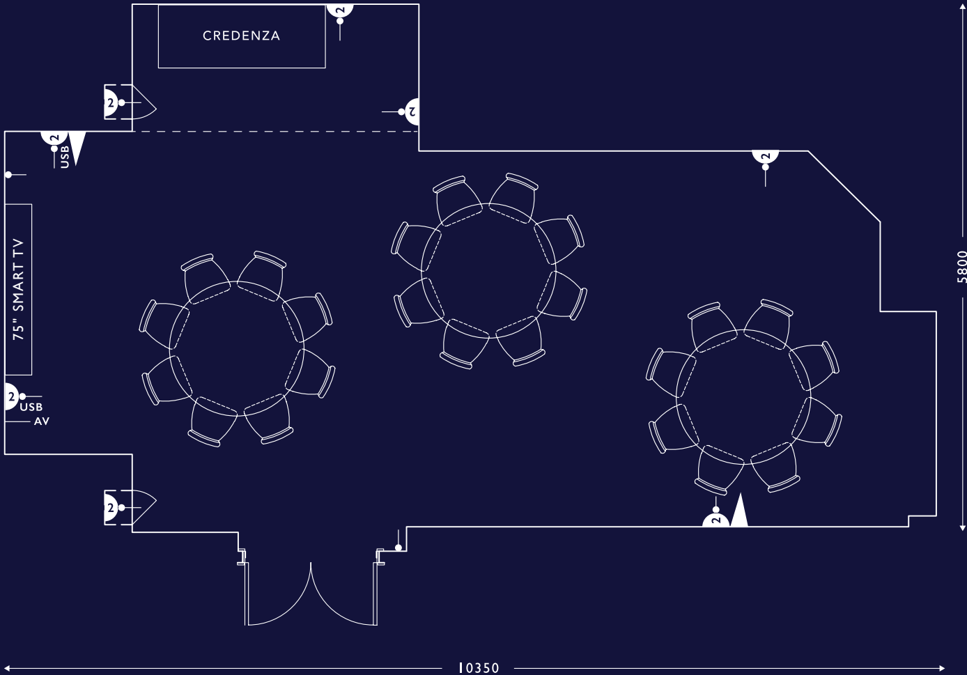
PRIVATE ROOM 5
